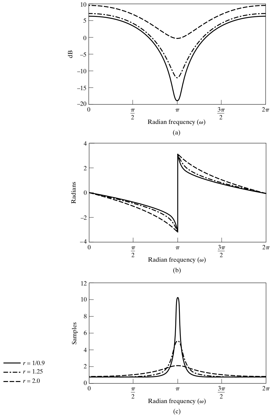
Figure 5.13 Frequency response for a single real zero outside the unit circle, with \theta = \pi , r = 1/0.9, 1.25, 2.0 . (a) Log magnitude. (b) Phase (principal value). (c) Group delay.
