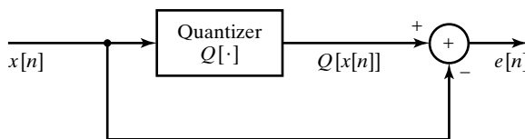
Figure 10.25 Procedure for obtaining quantization noise sequence.
