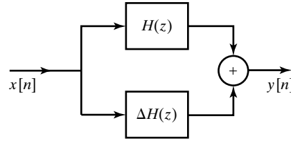
Figure 6.45 Representation of coefficient quantization in FIR systems.
