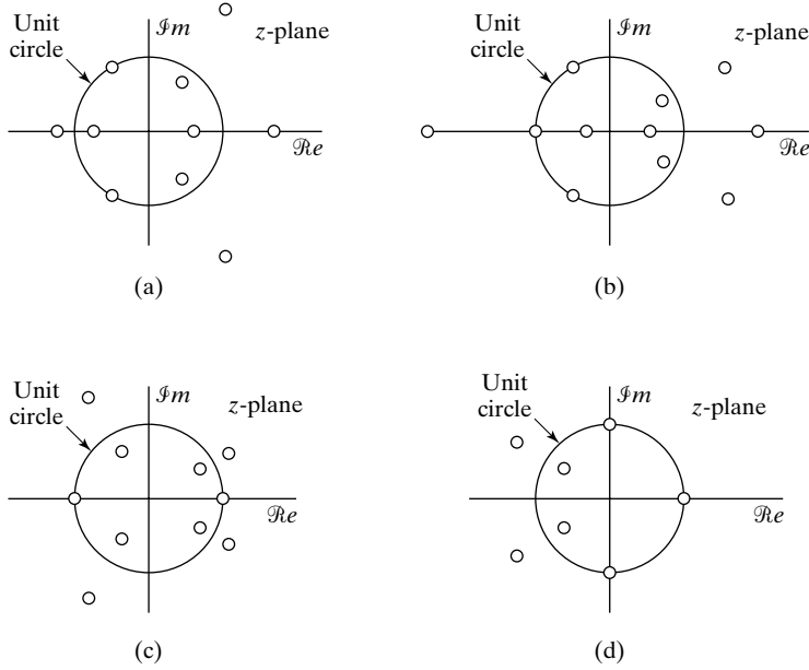
Figure 5.41 Typical plots of zeros for linear-phase systems. (a) Type I. (b) Type II. (c) Type III. (d) Type IV.
