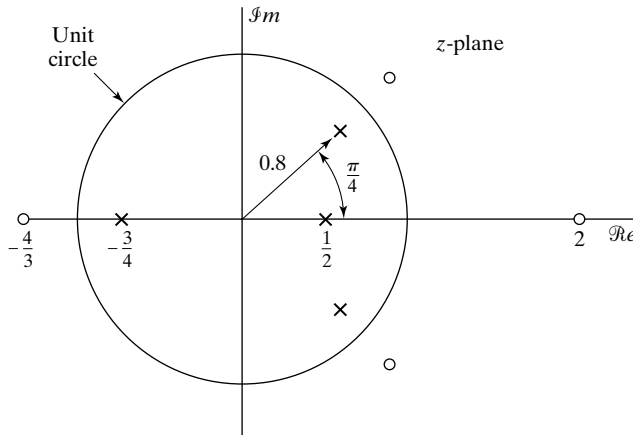
Figure 5.21 Typical pole-zero plot for an all-pass system.
