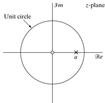
Figure 5.5 Pole-zero plot for Example 5.6.
