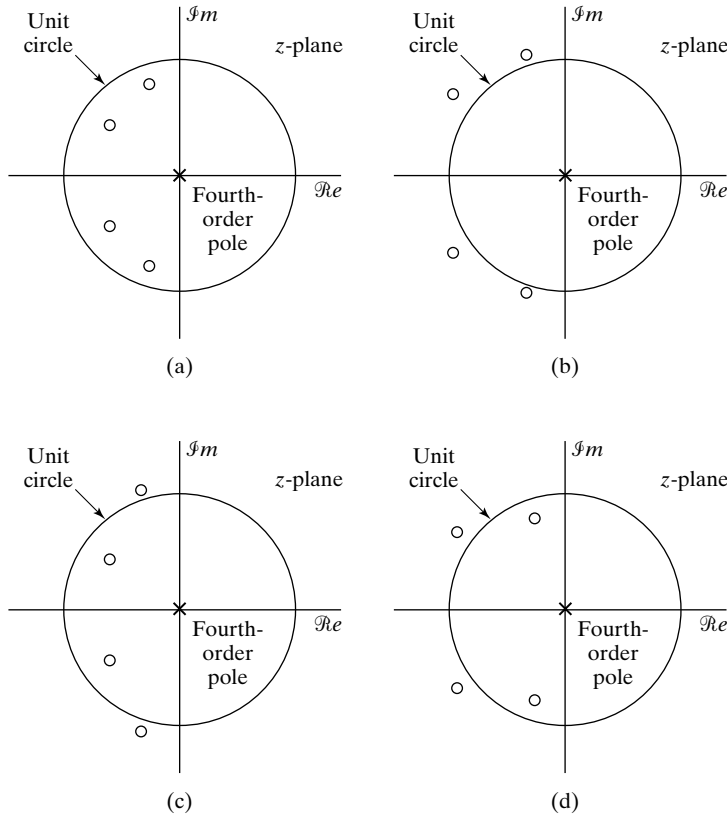
Figure 5.30 Four systems, all having the same frequency-response magnitude. Zeros are at all combinations of 0.9e^{j0.6\pi} and 0.8e^{j0.8\pi} and their reciprocals.
