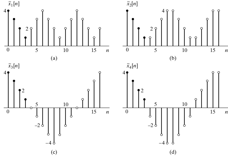
Figure 8.25 Four ways to extend a four-point sequence x[n] both periodically and symmetrically. The finite-length sequence x[n] is plotted with solid dots. (a) Type-1 periodic extension for DCT-1. (b) Type-2 periodic extension for DCT-2. (c) Type-3 periodic extension for DCT-3. (d) Type-4 periodic extension for DCT-4.
