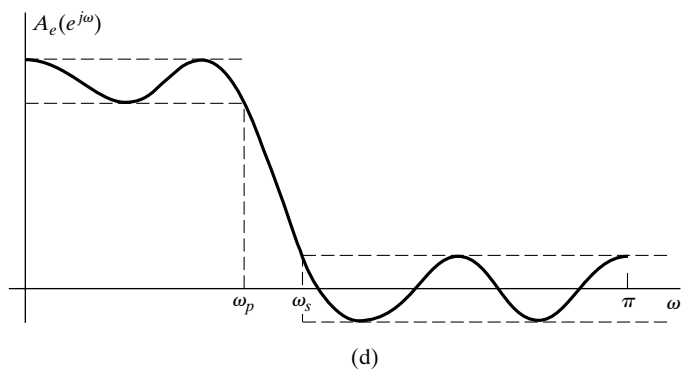
Figure 7.37 Possible optimum lowpass filter approximations for L = 7 . (a) L + 3 alternations (extraripple case). (b) L + 2 alternations (extremum at \omega = \pi ). (c) L + 2 alternations (extremum at \omega = 0 ). (d) L + 2 alternations (extremum at both \omega = 0 and \omega = \pi ).
