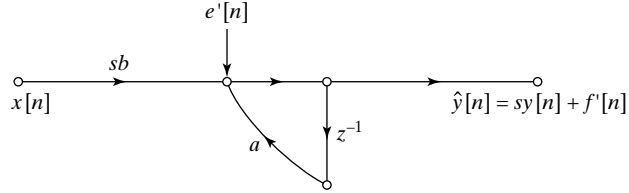
Figure 6.55 Scaled first-order system.
