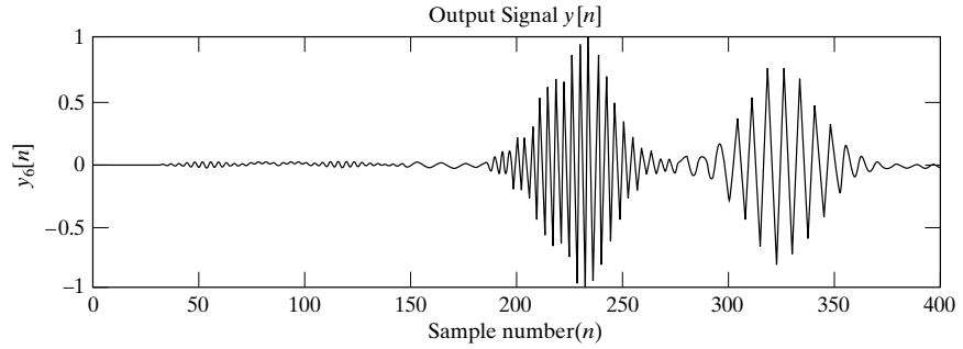
Figure 5.3 Output signal for Example 5.1.
