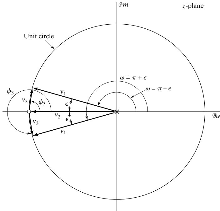
Figure 5.12 z -plane vectors for a zero at z = -1 for two different frequencies close to \pi ( \omega = \pi - \epsilon and \pi + \epsilon ).
