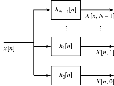
Figure 10.14 Filter bank representation of the time-dependent Fourier transform.
