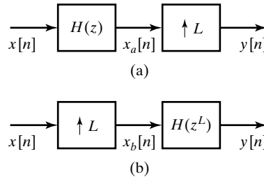
Figure 4.31 Two equivalent systems based on upsampling identities.
