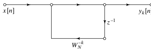
Figure 9.1 Flow graph of first-order complex recursive computation of X[k] .
