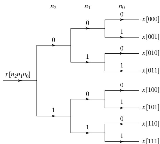
Figure 9.12 Tree diagram depicting normal-order sorting.
