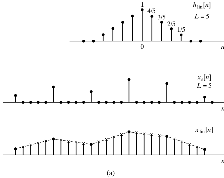
Figure 4.26 Impulse response for linear interpolation.
