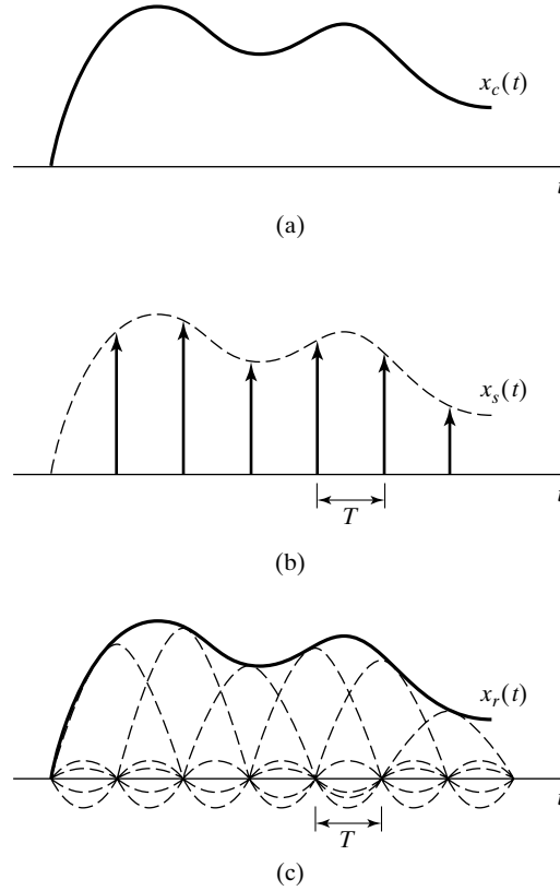
Figure 4.9 Ideal bandlimited interpolation.
