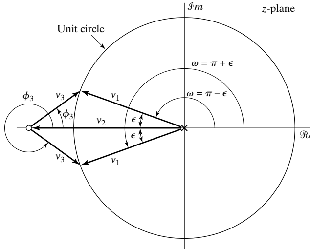
Figure 5.14 z -plane vectors for a single zero evaluated on the unit circle, with \theta = \pi , r > 1 .
