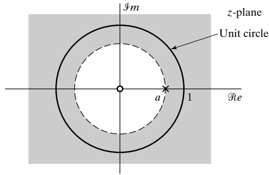
Figure 3.3 Pole-zero plot and region of convergence for Example 3.1.
