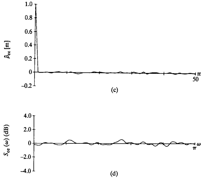
Figure 10.28 (continued) (c) Normalized autocorrelation estimate, 0 \leq m \leq 50 . (d) Power spectrum estimate using Bartlett window with M = 50 .
