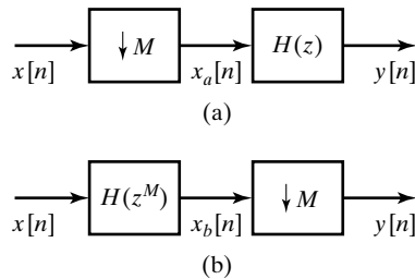
Figure 4.30 Two equivalent systems based on downsampling identities.
