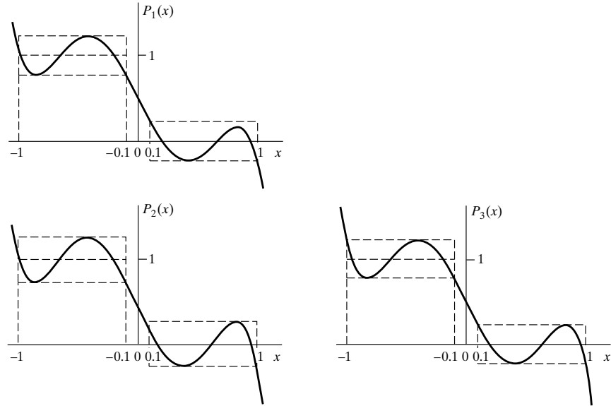
Figure 7.34 Fifth-order polynomials for Example 7.11.
