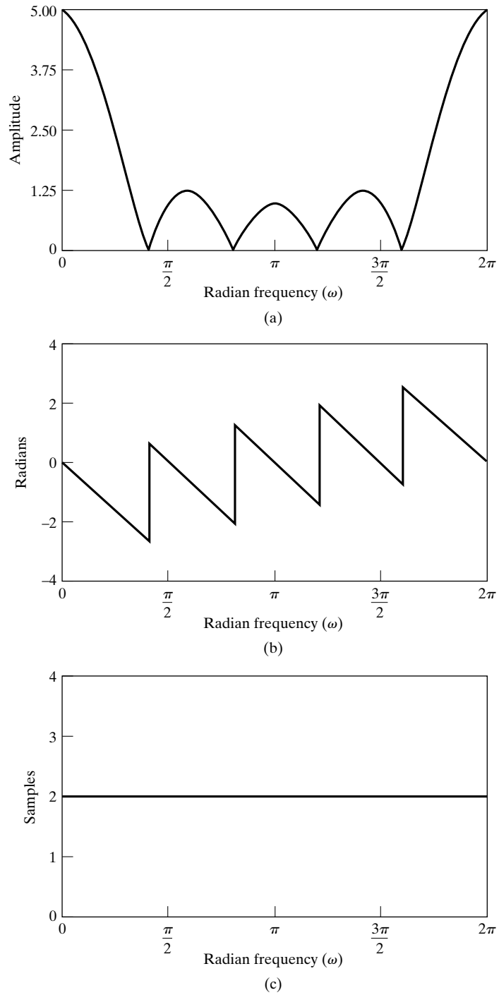
Figure 5.37 Frequency response of type I system of Example 5.17. (a) Magnitude. (b) Phase. (c) Group delay.
