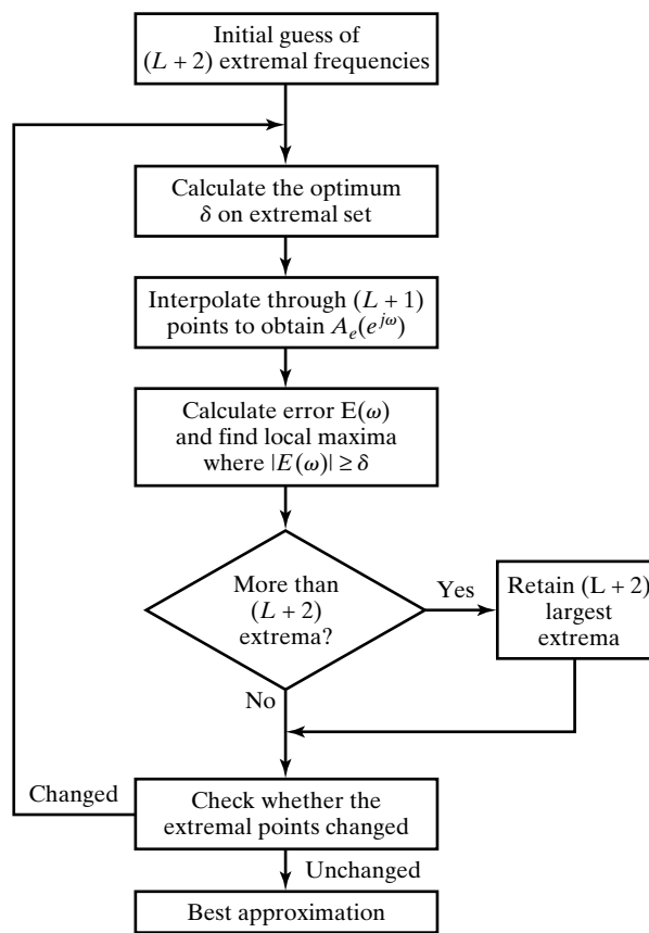
Figure 7.41 Flowchart of Parks–McClellan algorithm.
