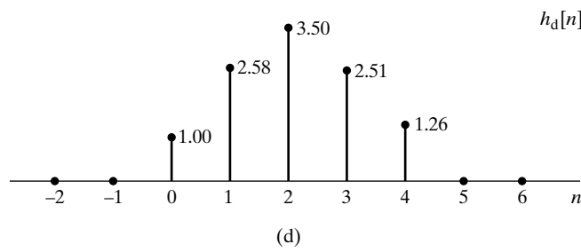
Figure 5.31 Sequences corresponding to the pole-zero plots of Figure 5.30.
