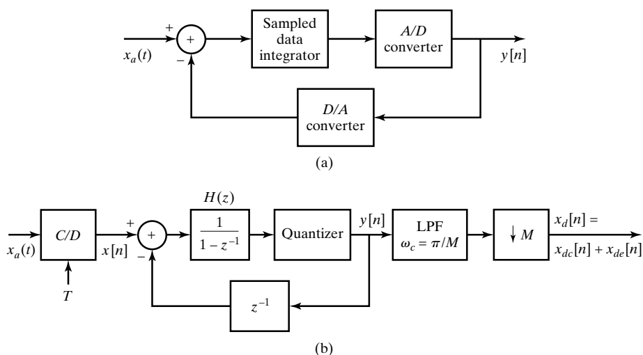
Figure 4.61 Oversampled quantizer with noise shaping.
