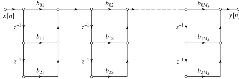
Figure 6.33 Cascade-form realization of an FIR system.
