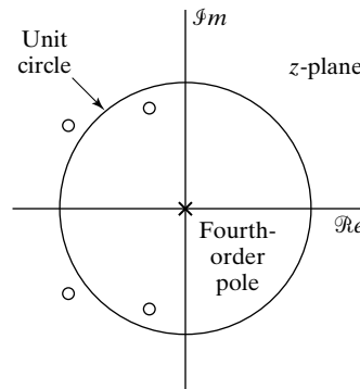
Figure 5.26 Pole-zero plot of FIR system in Example 5.15.
