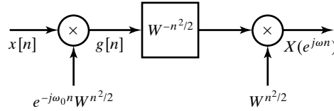
Figure 9.26 Block diagram of chirp transform algorithm.
