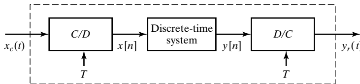
Figure 4.11 Discrete-time processing of continuous-time signals.
