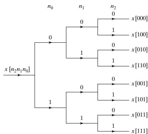
Figure 9.13 Tree diagram depicting bit-reversed sorting.
