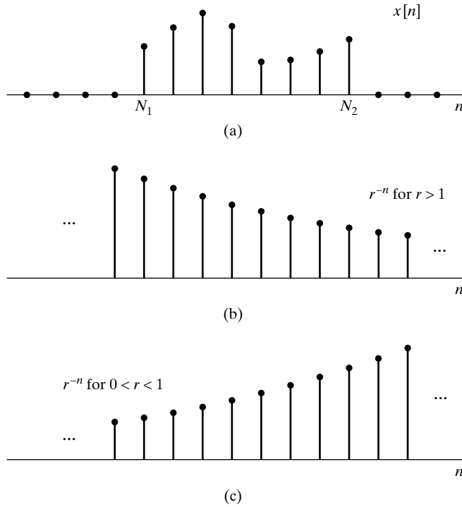
Figure 3.8 Finite-length sequence and weighting sequences implicit in convergence of the z-transform. (a) The finite-length sequence x[n] . (b) Weighting sequence r^{-n} for 1 < r . (c) Weighting sequence r^{-n} for 0 < r < 1 .
