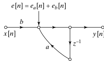
Figure 6.52 First-order linear noise model.
