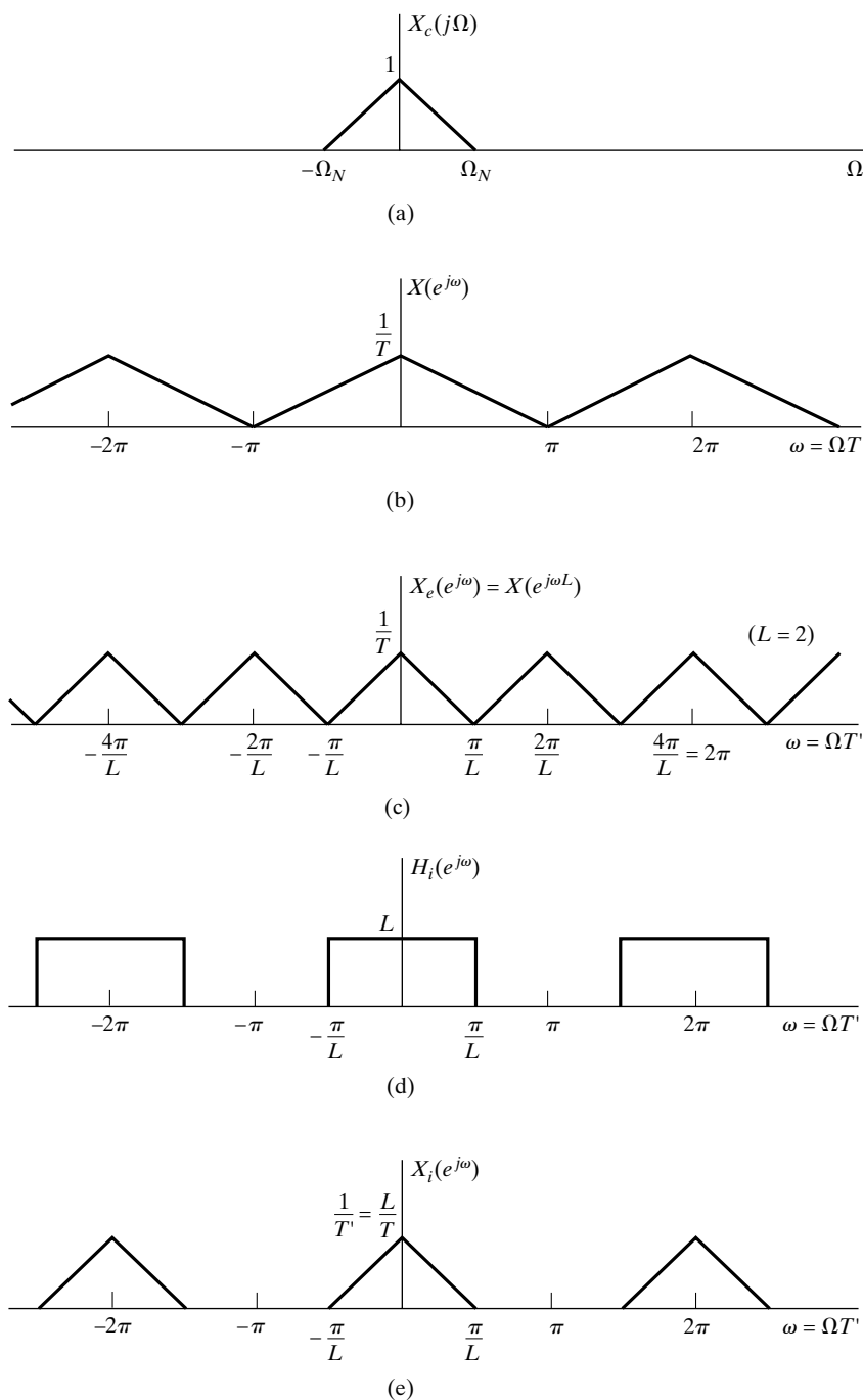
Figure 4.25 Frequency-domain illustration of interpolation.
