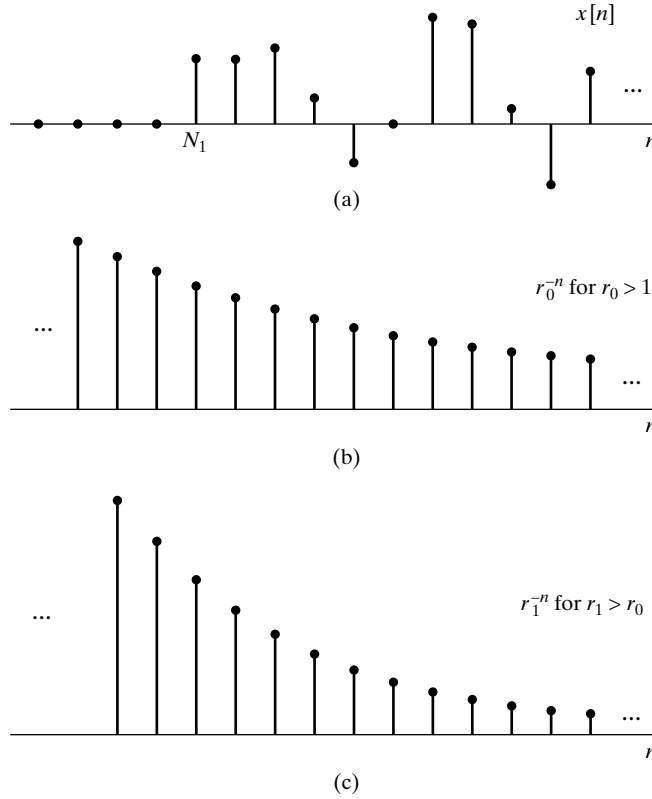
Figure 3.9 Right-sided sequence and weighting sequences implicit in convergence of the z-transform. (a) The right-sided sequence x[n] . (b) Weighting sequence r_0^{-n} for 1 < r_0 . (c) Weighting sequence r_1^{-n} for r_1 > r_0 .
