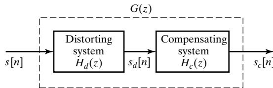
Figure 5.25 Illustration of distortion compensation by linear filtering.
