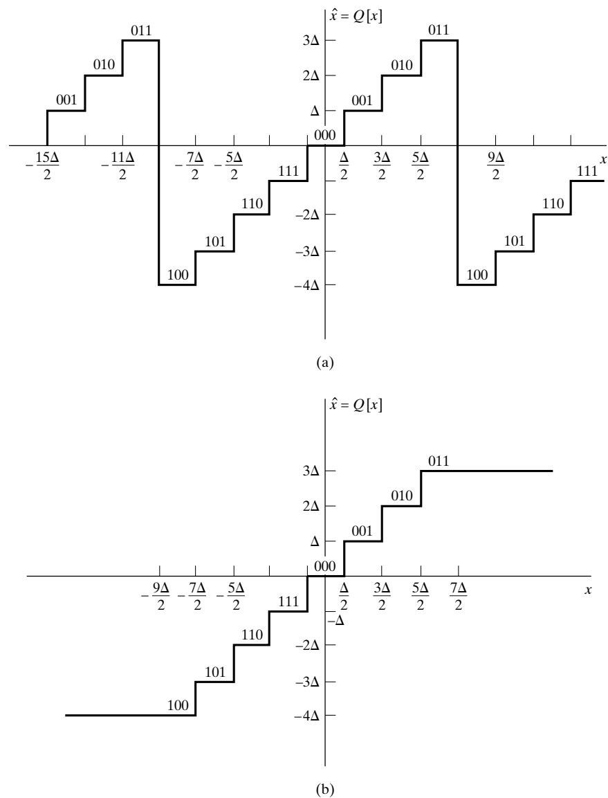
Figure 6.38 Two's-complement rounding. (a) Natural overflow. (b) Saturation.
