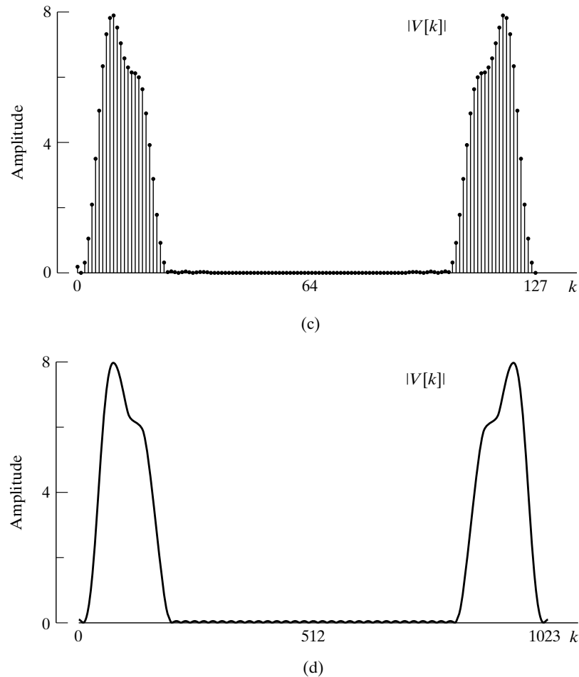
Figure 10.9 (continued) (c) Magnitude of DFT for N = 128 . (d) Magnitude of DFT for N = 1024 . (DFT values are linearly interpolated to obtain a smooth curve.)
