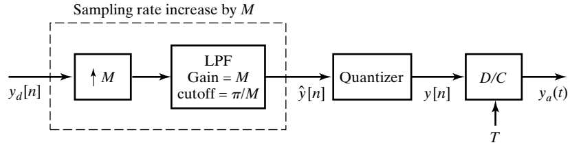
Figure 4.67 Oversampled D/A conversion.
