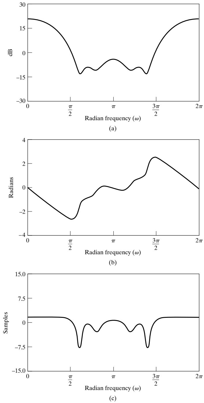
Figure 5.28 Frequency response for minimum-phase system in Example 5.15. (a) Log magnitude. (b) Phase. (c) Group delay.
