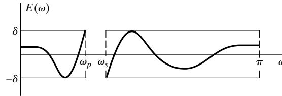
Figure 7.33 Weighted error for the approximation of Figure 7.32.
