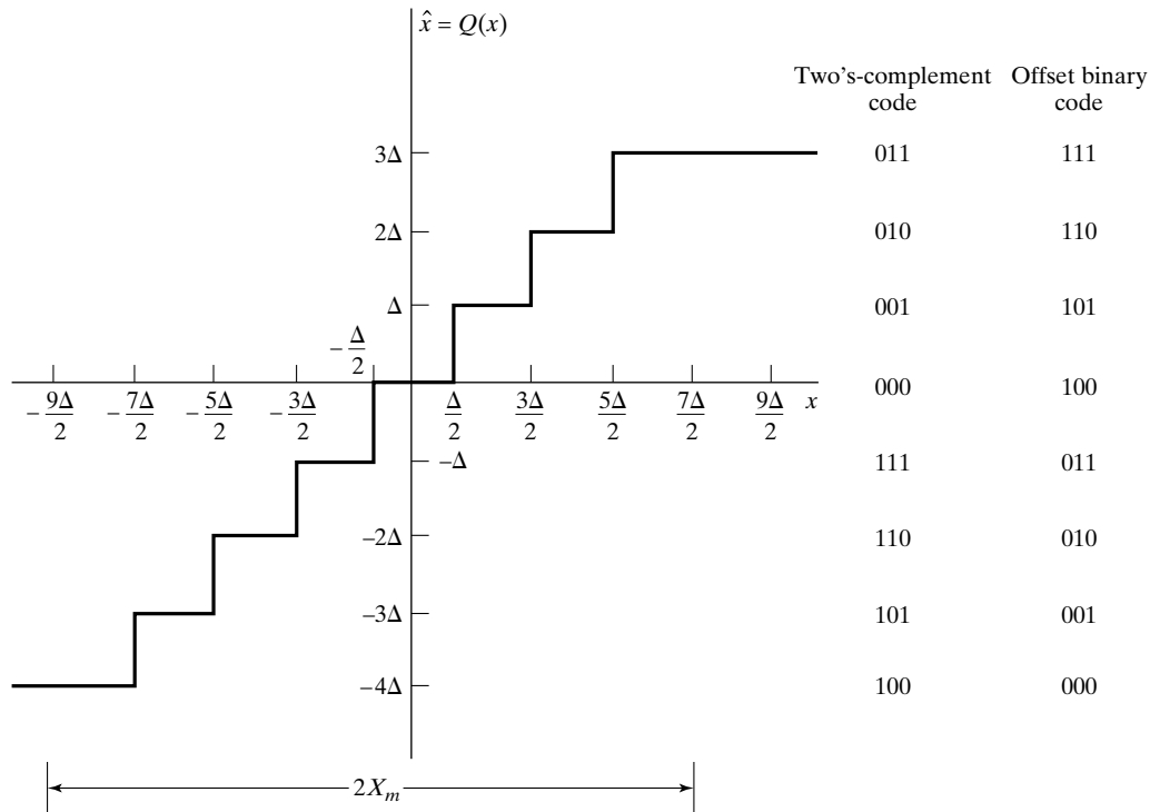
Figure 4.48 Typical quantizer for A/D conversion.
