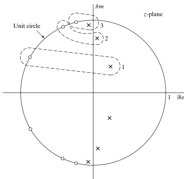
Figure 6.57 Pole-zero plot for sixth-order system of Figure 6.56, showing pairing of poles and zeros.
