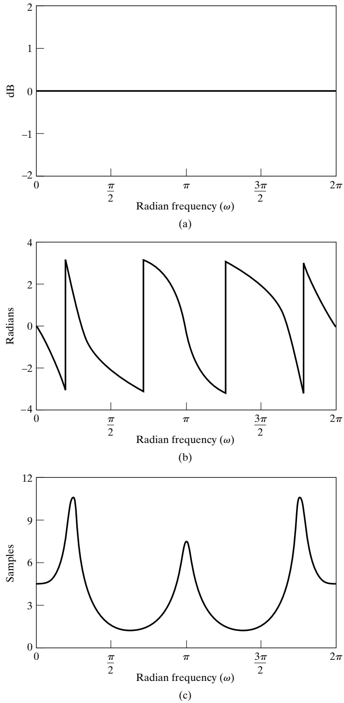
Figure 5.24 Frequency response for an all-pass system with the pole-zero plot in Figure 5.21. (a) Log magnitude. (b) Phase (principal value). (c) Group delay.
