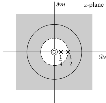
Figure 3.12 Pole-zero plot and ROC for Example 3.8.
