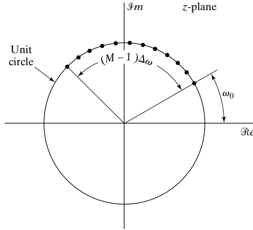
Figure 9.25 Frequency samples for chirp transform algorithm.
