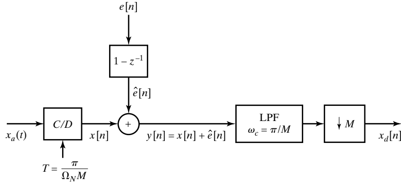
Figure 4.63 Equivalent representation of Figure 4.62.
