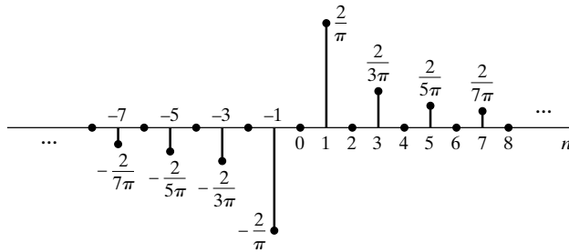
Figure 11.5 Impulse response of an ideal Hilbert transformer or 90-degree phase shifter.
