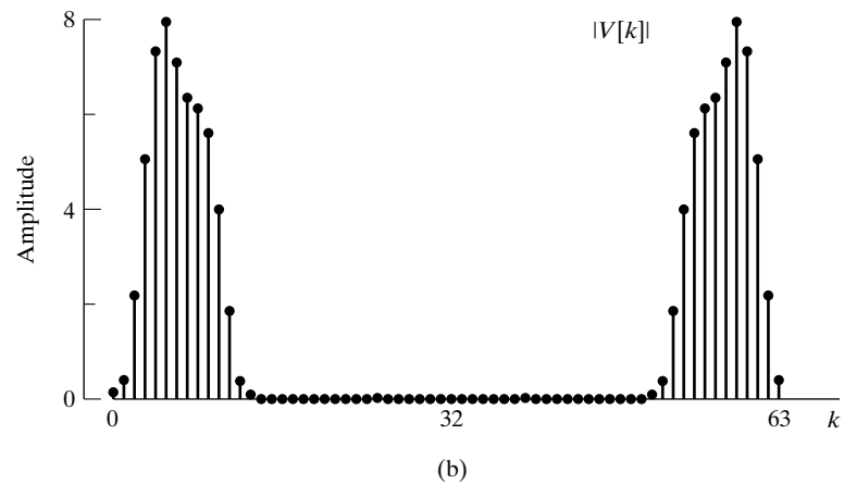
Figure 10.9 Illustration of effect of DFT length for Kaiser window of length L = 32 . (a) Magnitude of DFT for N = 32 . (b) Magnitude of DFT for N = 64 .
