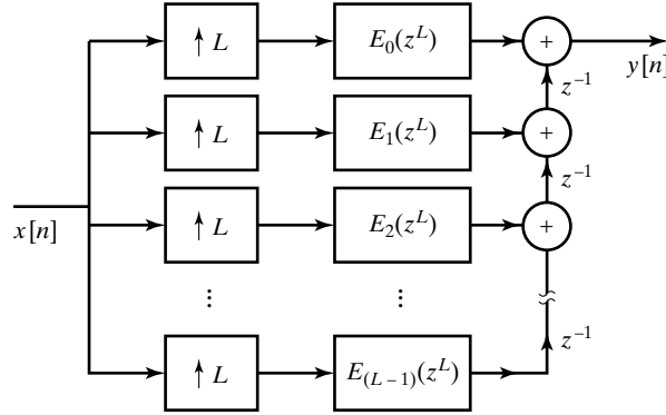
Figure 4.39 Implementation of interpolation filter using polyphase decomposition.
