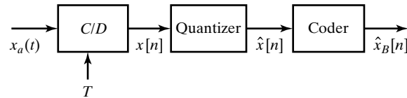
Figure 4.47 Conceptual representation of the system in Figure 4.45.
