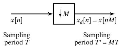
Figure 4.20 Representation of a compressor or discrete-time sampler.
