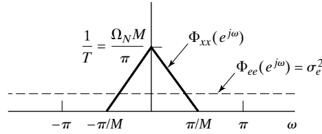
Figure 4.59 Power spectral density of signal and quantization noise with an oversampling factor of M .
