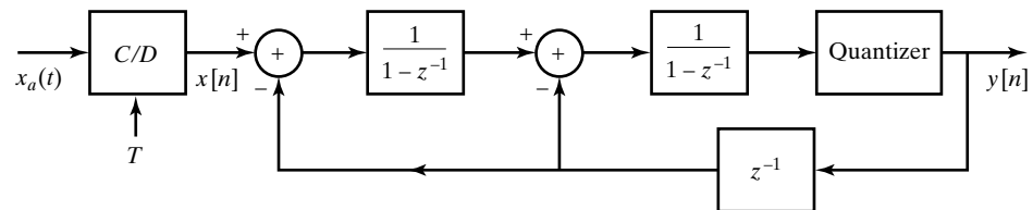
Figure 4.66 Oversampled quantizer with second-order noise shaping.
