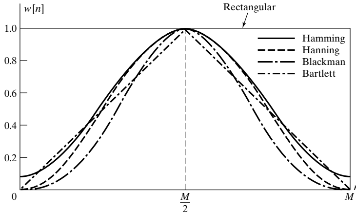
Figure 7.21 Commonly used windows.
