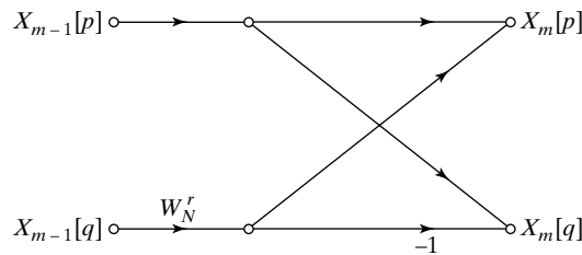
Figure 9.11 Flow graph of Eqs. (9.21).
