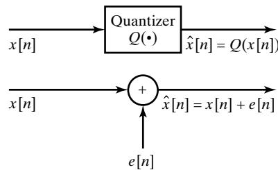
Figure 4.50 Additive noise model for quantizer.
