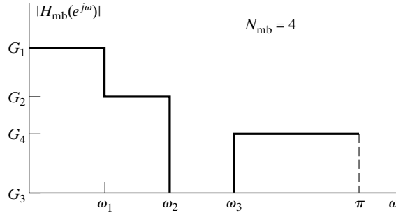
Figure 7.28 Ideal frequency response for multiband filter.
