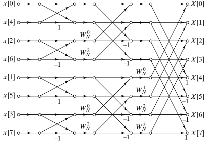
Figure 9.32 Flow graph for decimation-in-time FFT algorithm.
