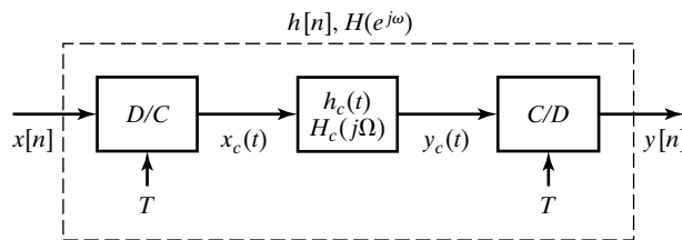
Figure 4.16 Continuous-time processing of discrete-time signals.
