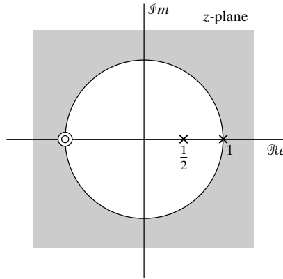
Figure 3.13 Pole-zero plot for the z-transform in Example 3.9.
