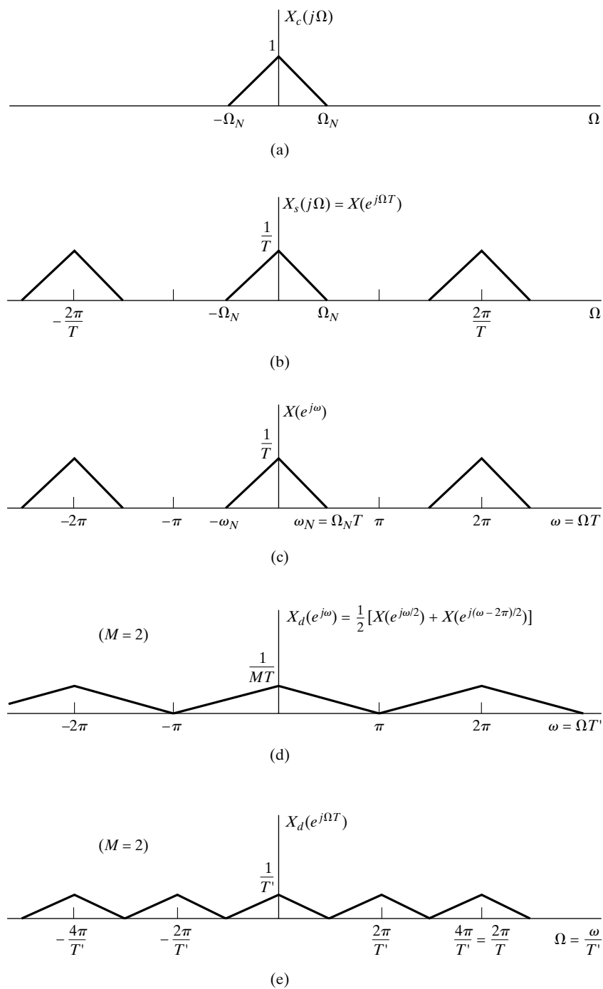
Figure 4.21 Frequency-domain illustration of downsampling.
