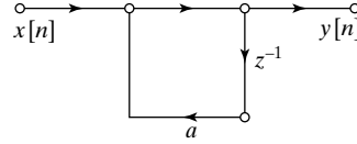
Figure 6.24 Flow graph of simple first-order system.
