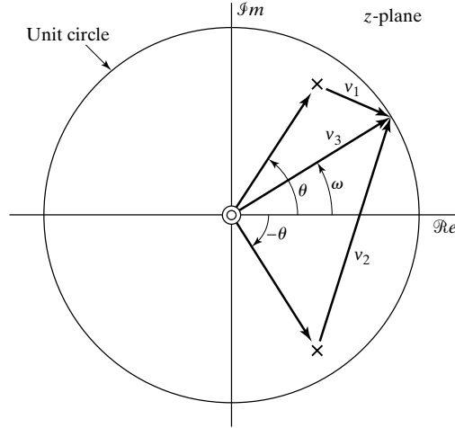
Figure 5.15 Pole-zero plot for Example 5.8.
