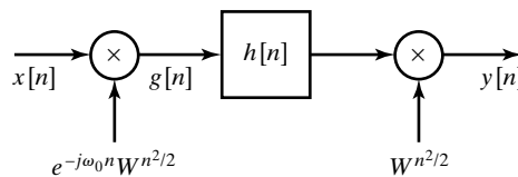
Figure 9.29 Block diagram of chirp transform system for finite-length impulse response.
