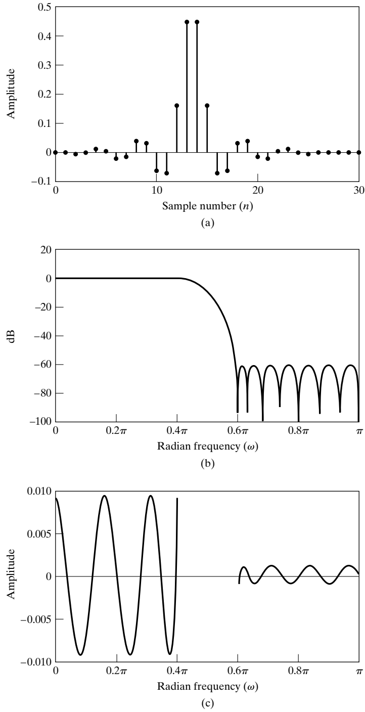
Figure 7.44 Optimum type II FIR lowpass filter for \omega_p = 0.4\pi , \omega_s = 0.6\pi , K = 10 , and M = 27 . (a) Impulse response. (b) Log magnitude of frequency response. (c) Approximation error (unweighted).
