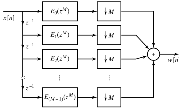
Figure 4.36 Implementation of decimation filter using polyphase decomposition.
