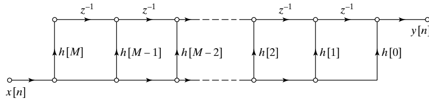
Figure 6.32 Transposition of the network of Figure 6.31.
