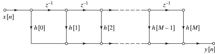
Figure 6.31 Direct-form realization of an FIR system.
