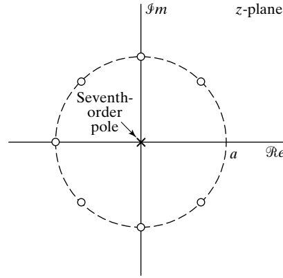
Figure 5.6 Pole-zero plot for Example 5.7.
