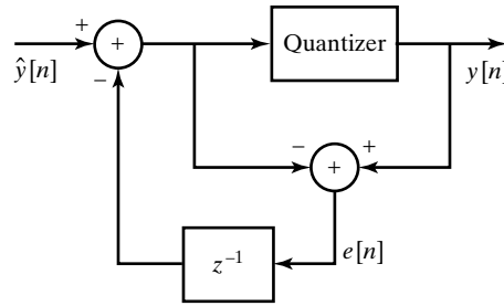
Figure 4.68 First-order noise-shaping system for oversampled D/A quantization.
