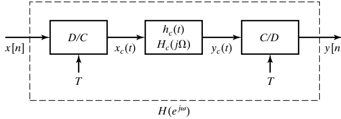
Figure 5.33 Interpretation of noninteger delay in discrete-time systems.
