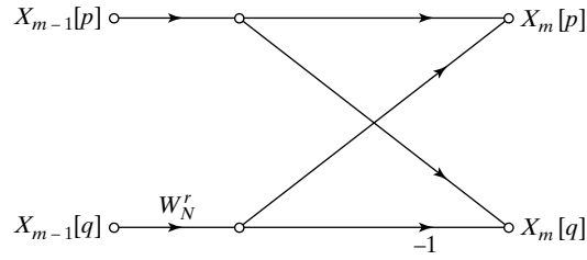
Figure 9.33 Butterfly computation for decimation in time.
